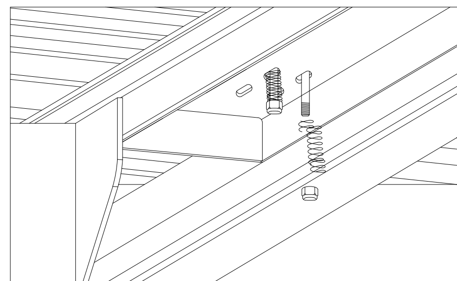
Figure 9.2: Spring Installation
