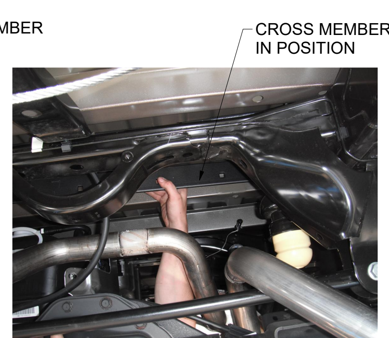
Figure 5.4: As viewed from rear towards axle.
