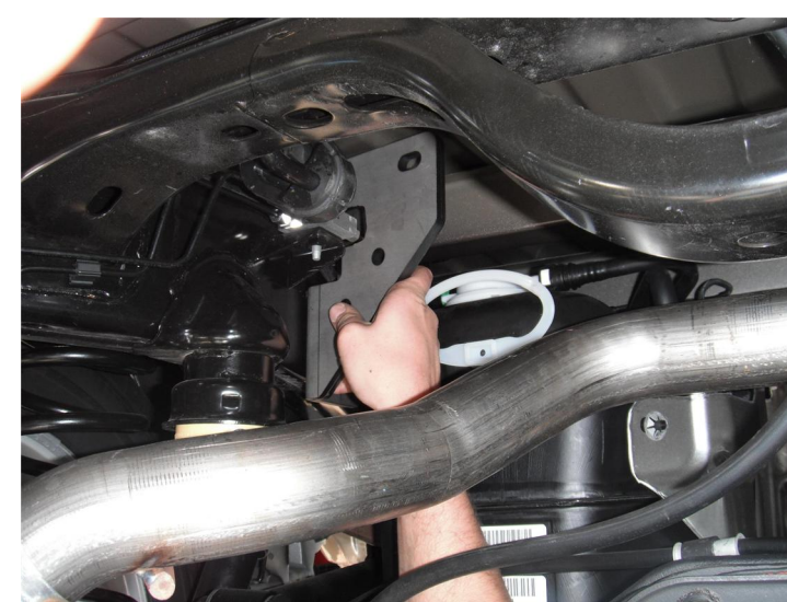
Figure 6.5: Driver side plate as viewed from floor up toward driver side frame. (Fuel tank is not shown.)
