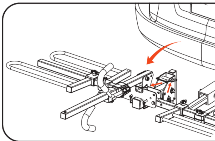
Detail R
