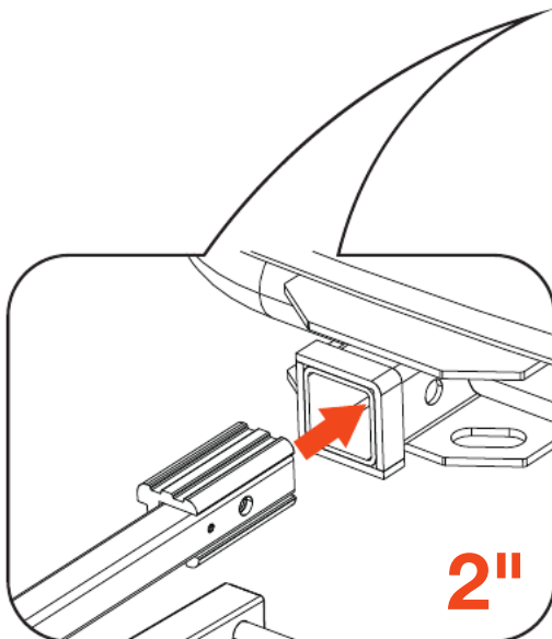
Detail J
