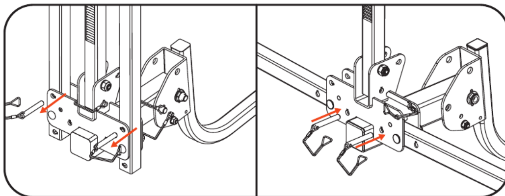
Detail D
