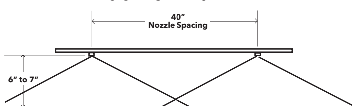
Flat Uniform Sprayer Pattern
