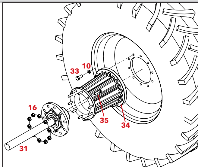
VIEW A
