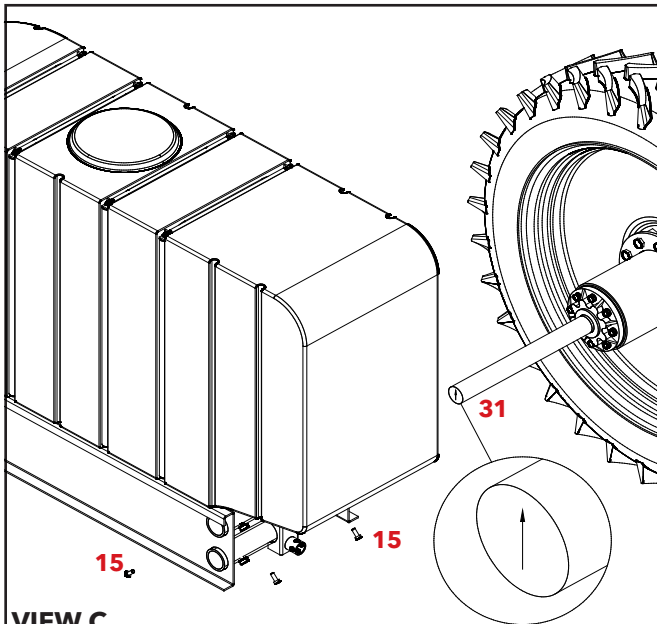
VIEW C
