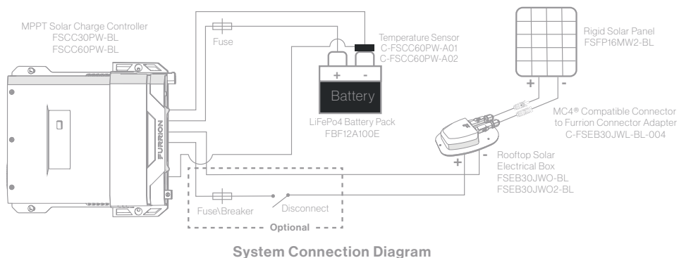
System Connection Diagram
