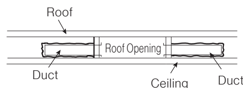
SIDE VIEW (TOWARD BACK OF RV)
