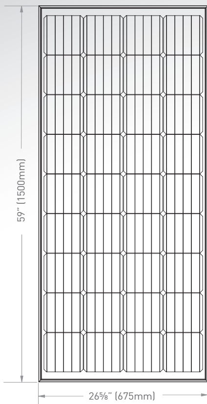
Front View
