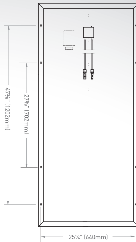
Back View
