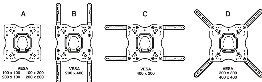
Furrion Aurora™ TV VESA MOUNTING PATTERN
