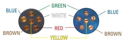
TRAILER END As viewed from core back side where wires are attached with screws.
