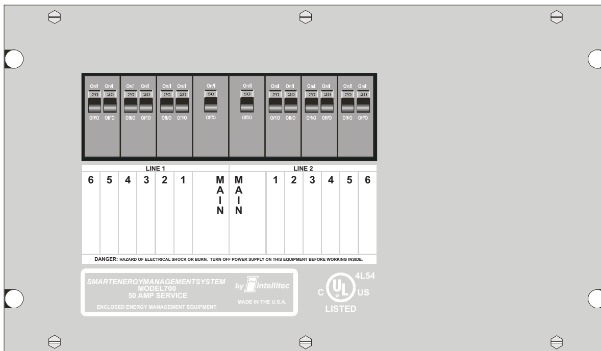
100 Amp EMS Distribution Panel
