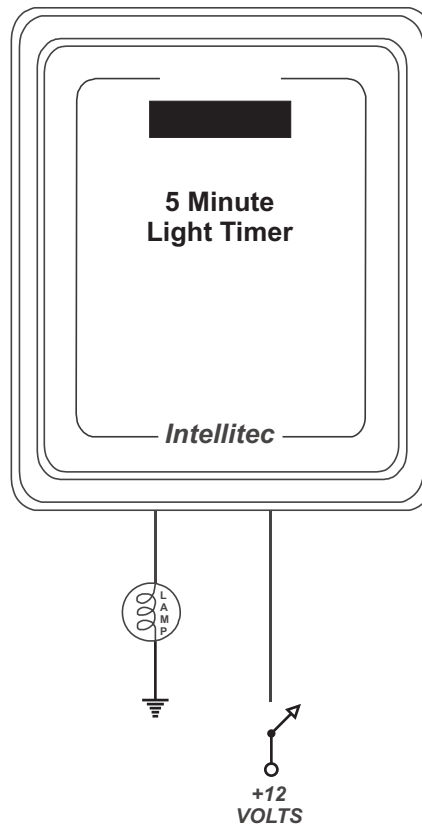
HIGH SIDE CONNECTION
