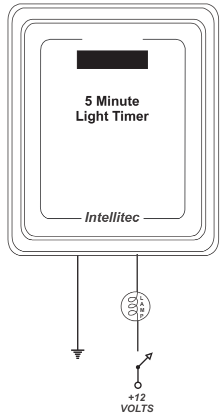
LOW SIDE CONNECTION
