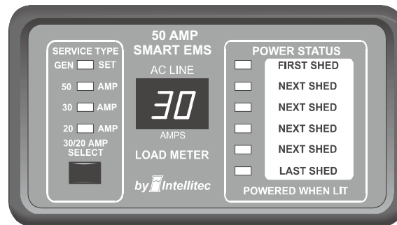
50 Amp EMS Display Panel
