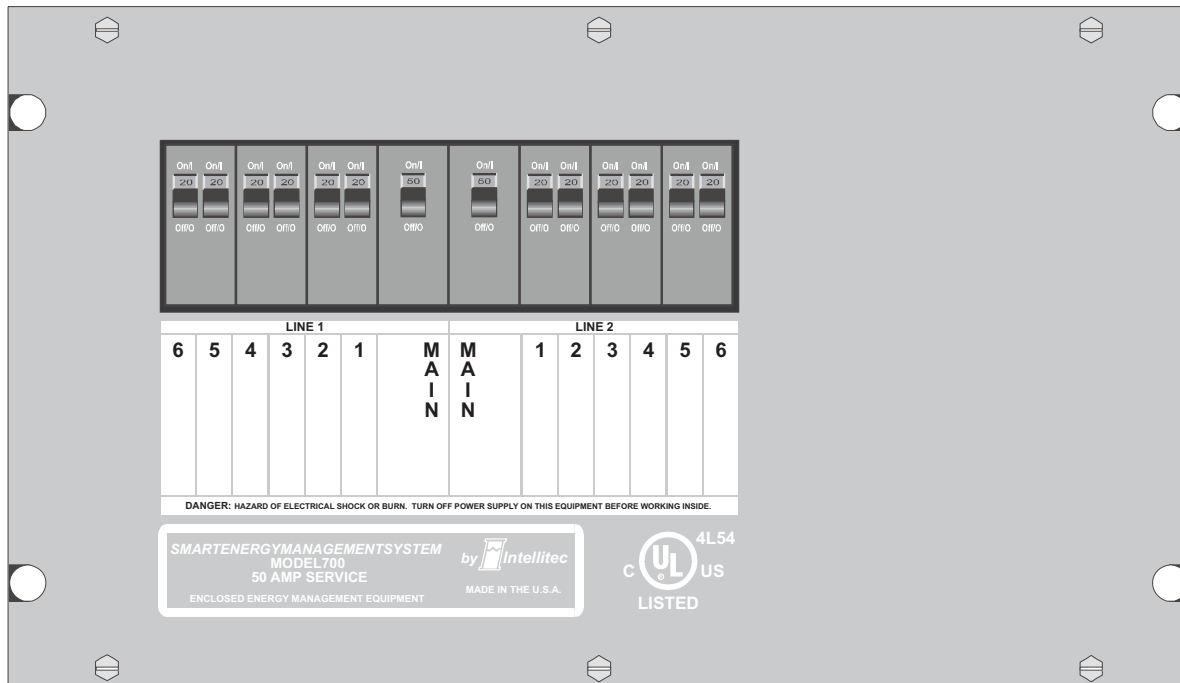
50 Amp EMS Distribution Panel
