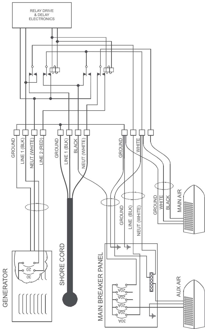
TYPICAL 30 AMP SERVICE CONNECTIONS
