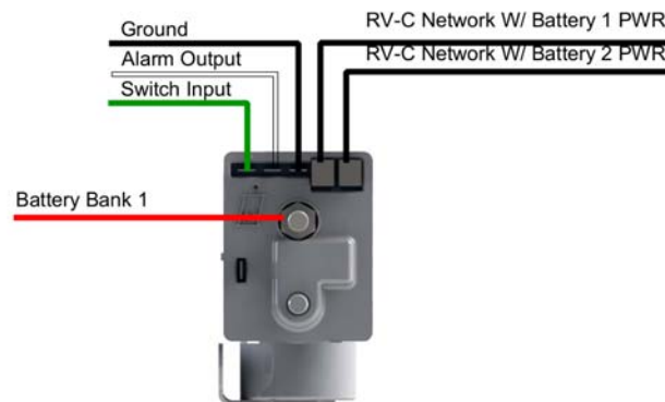
Wire Diagram 2
