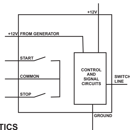
EQUIVALENT CIRCUIT
