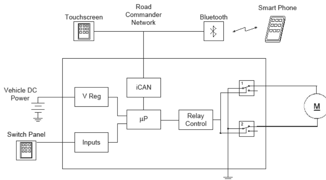
Typical Arrangement – Single Slide Out Control Interface
