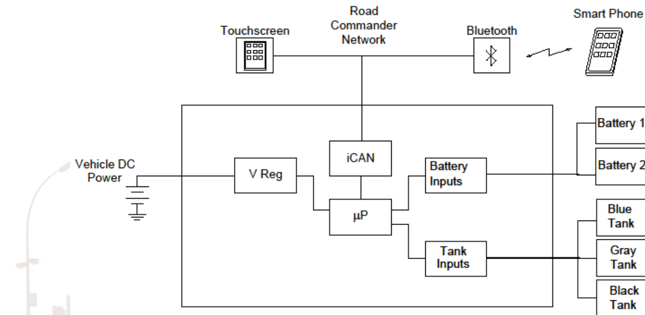
Typical Arrangement – 2 Battery Banks, 3 Tanks
