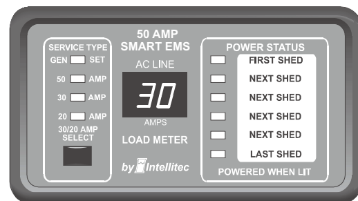
50 Amp EMS Display Panel P/N 00-00684-100
