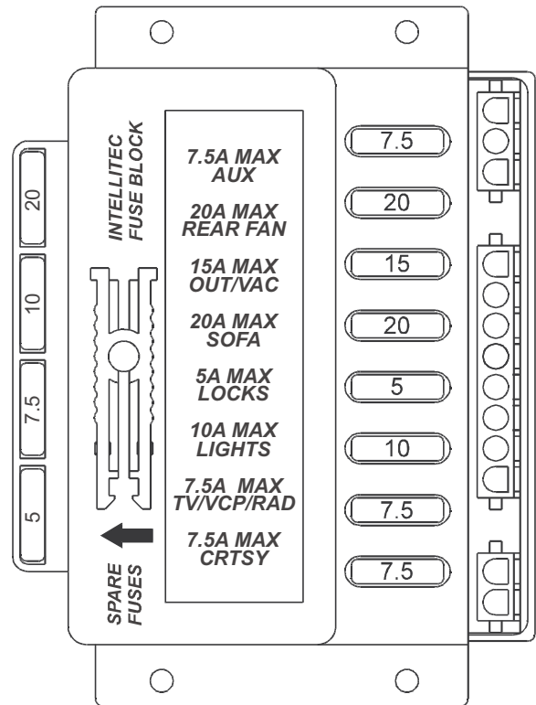
Part Number 00-00344-000
