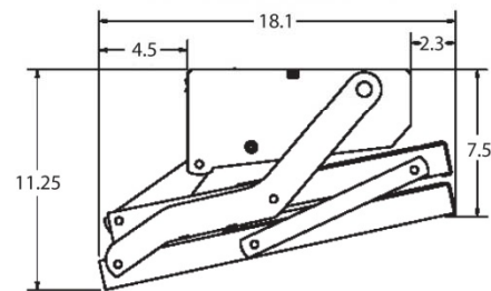
RETRACTED PROFILE
