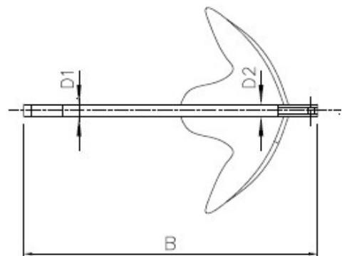
BASIC DIMENSIONS OF ST/ST CLAW ANCHOR
