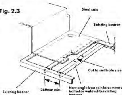
Typical application for Steel cockpits
