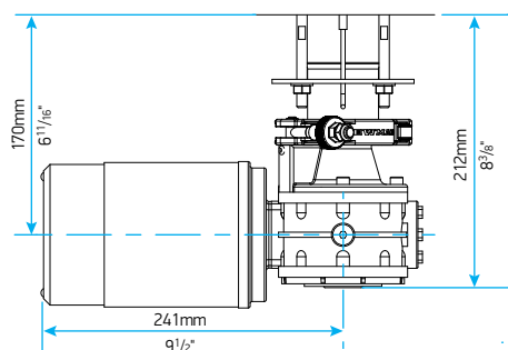
V1 Motor Gearbox (with FastFit™ feature)
