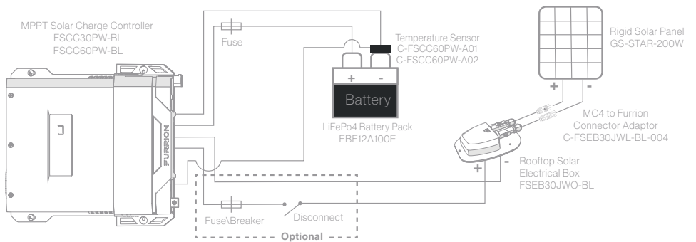
System Connection Diagram
