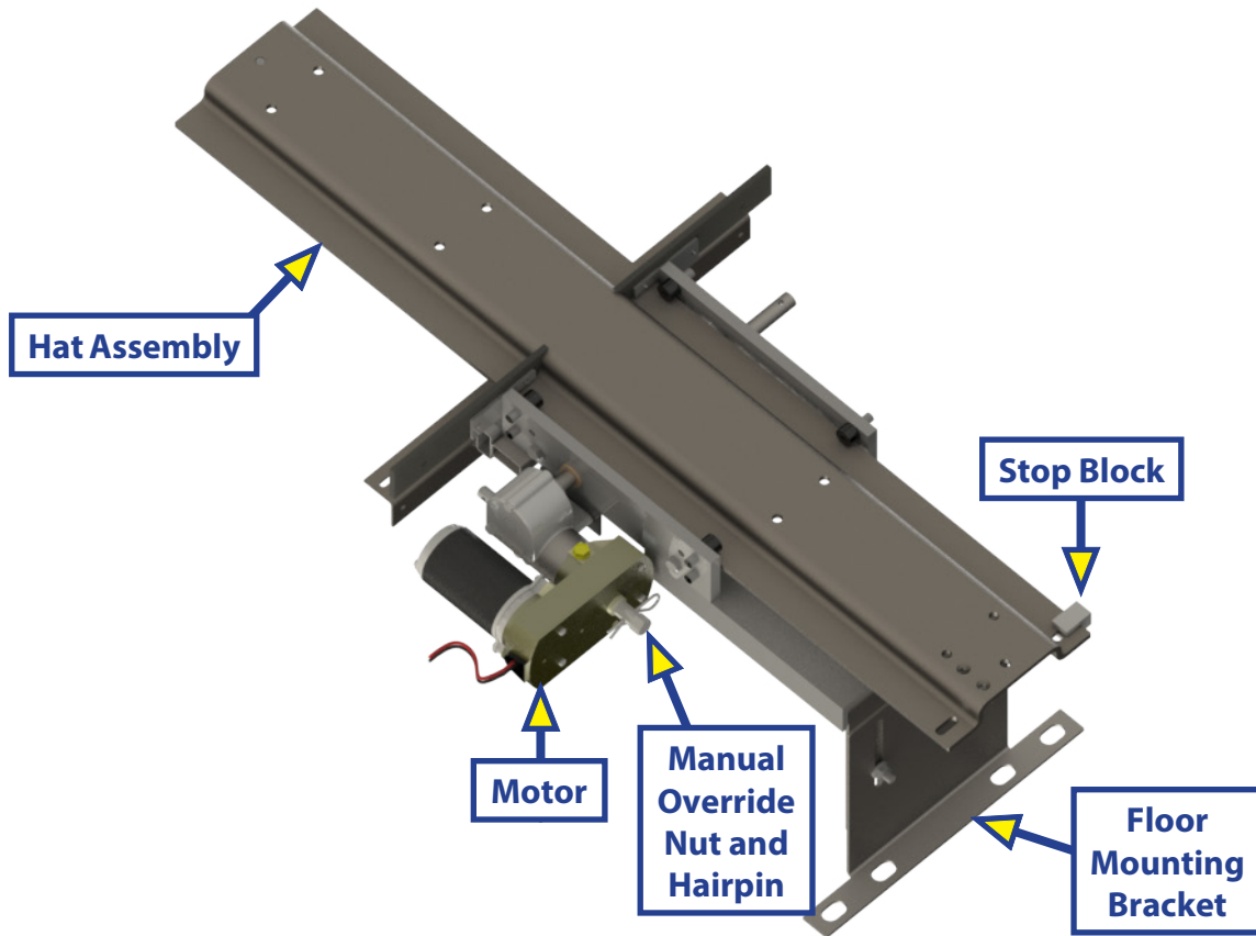
Topside View
