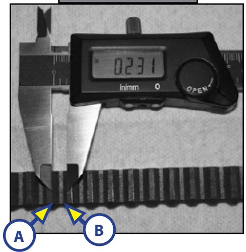
Fig. 3.2 - 20° Rack
