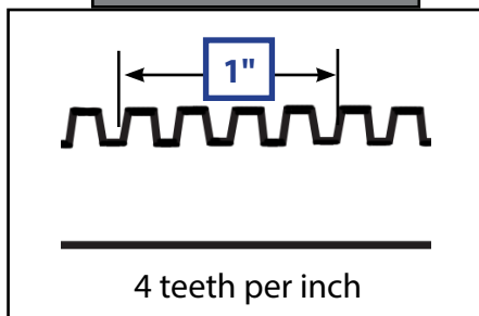
Fig. 2.2 - 14.5° Rack
