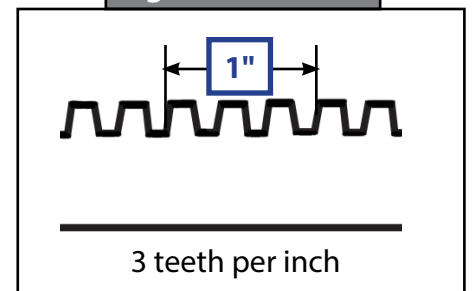
Fig. 3.2 - 20° Rack
