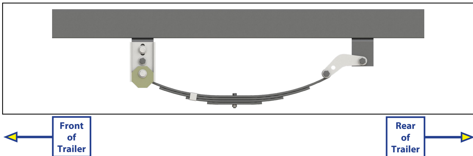
Single Axle Set-up
