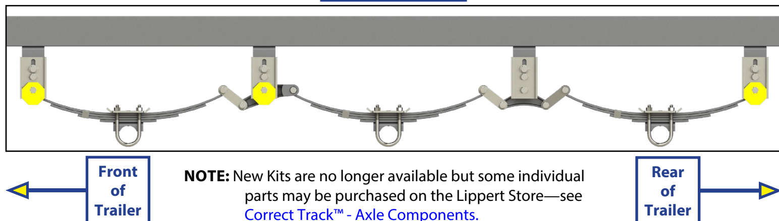
Triple Axle Set-Up
