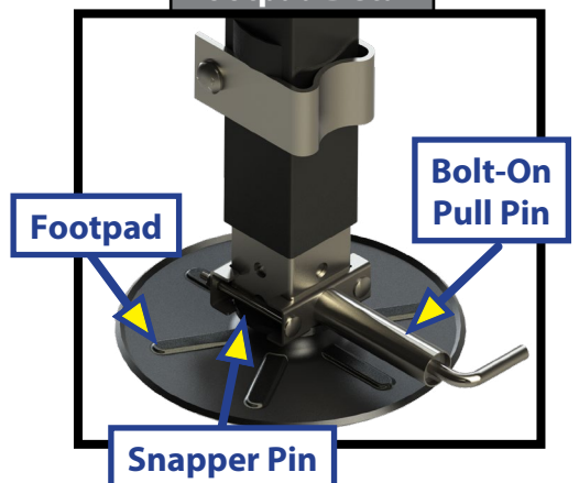
Footpad Detail
