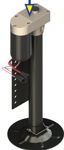
Right Hall Effect Jacks; Rear and Middle x2
