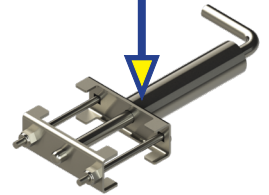
Carriage Bolt/ Nut x4
