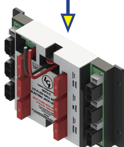
6 Point Controller
