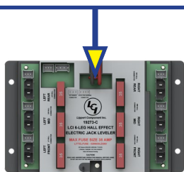
6 Point Controller
