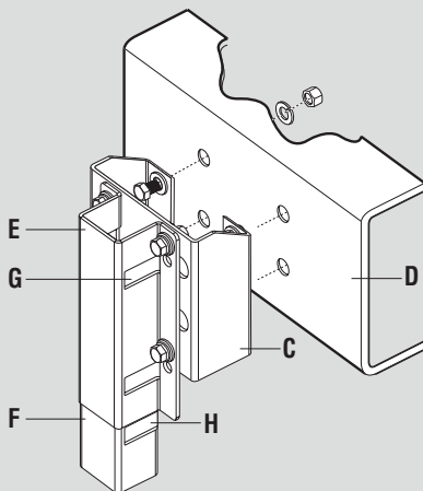
Figure 12 — 7.5K Square Tube
