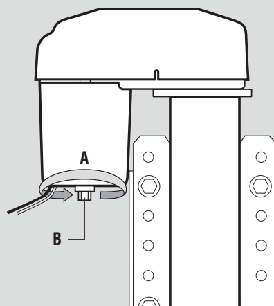
Figure 10 — Manual Override
