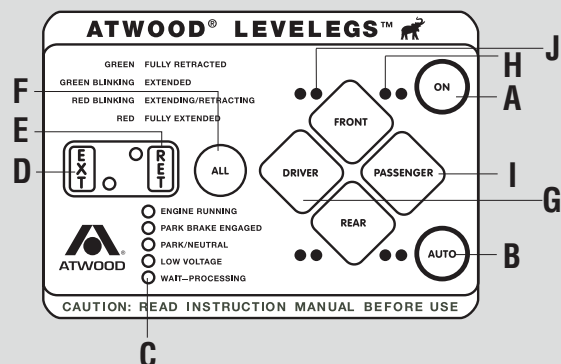
Figure 9 — Control Pad
