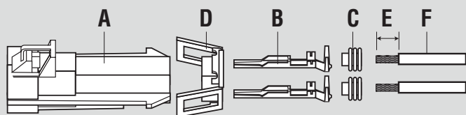
Figure 6 — Delphi Connector
