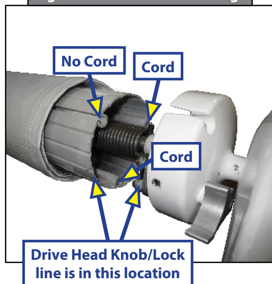
Fig. 2 - Flat or Pitched Awnings
