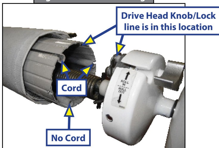
Fig. 3 - Short Arm Awnings
