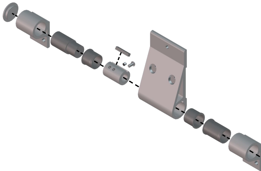
Fig. 16 - Assembly A
