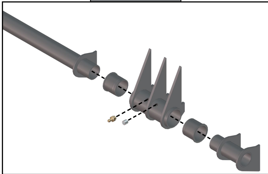
Fig. 8 - Assembly A
