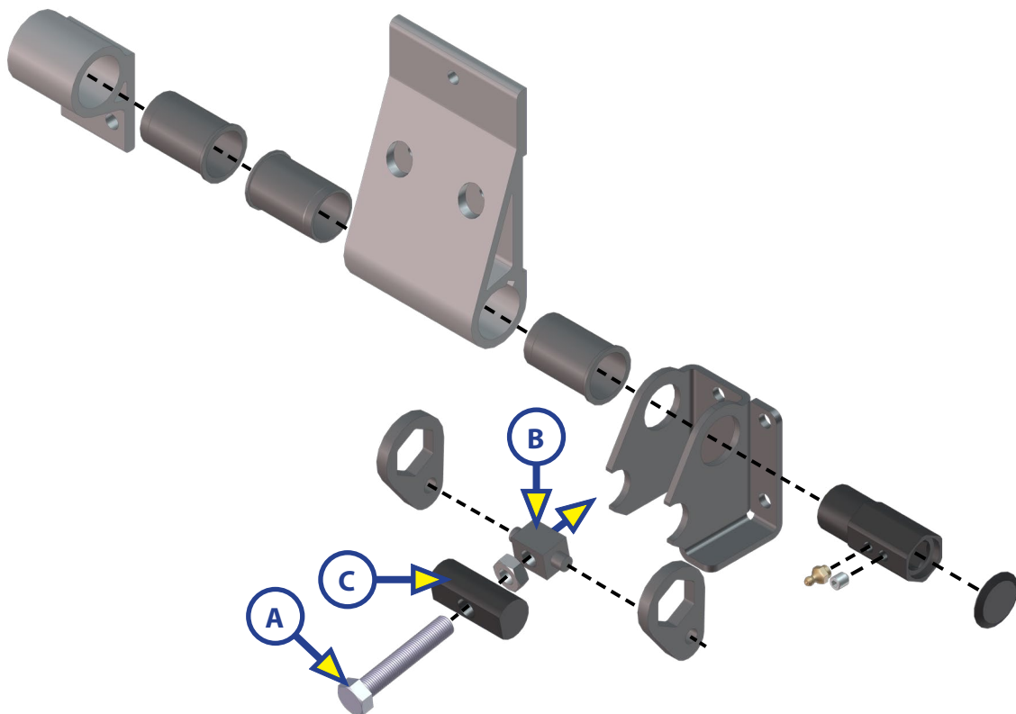
Fig. 17 - Assembly B
