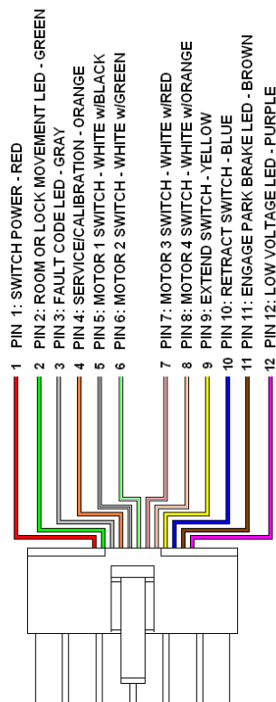
Control to Touch Pad Harness 1510000195
