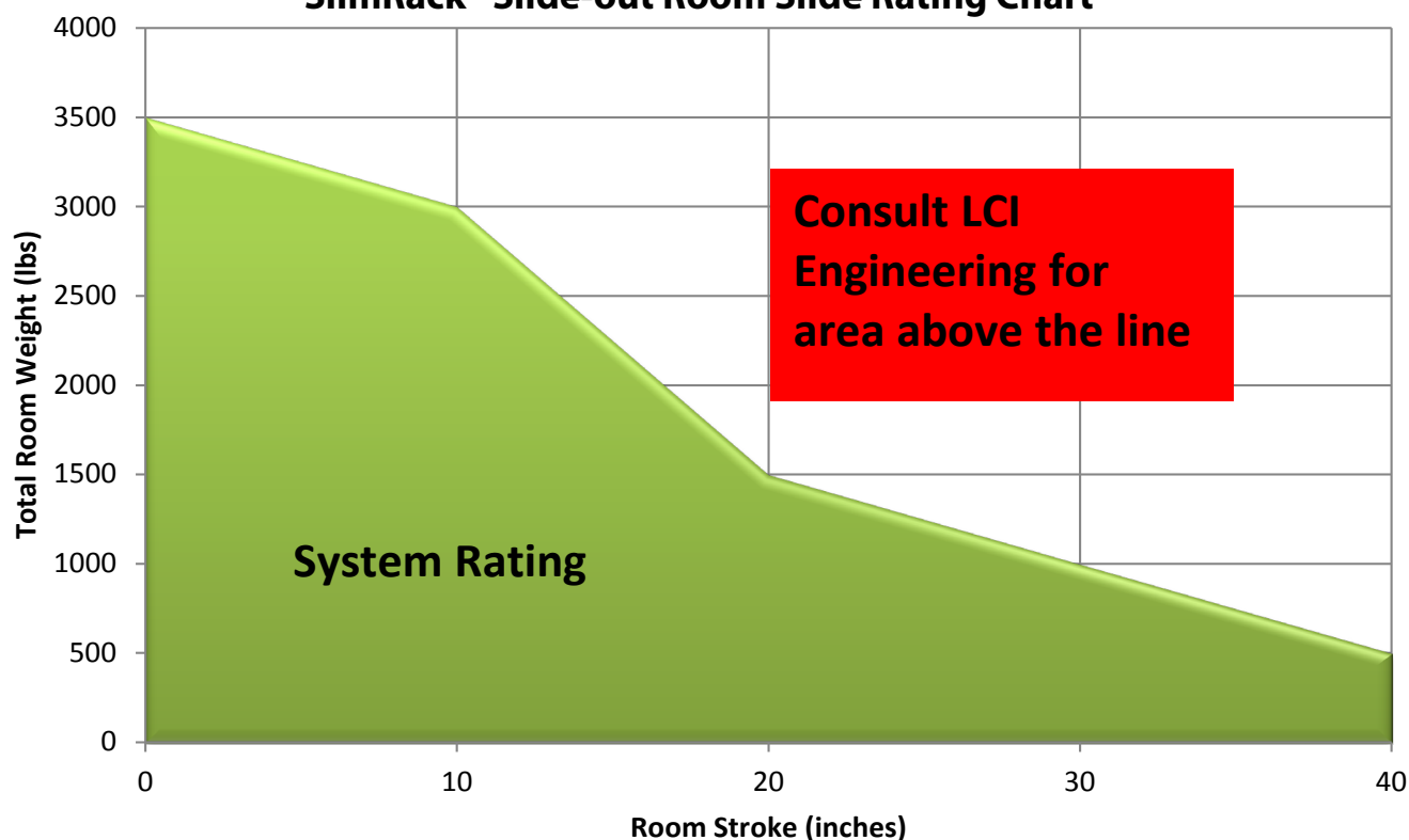
SlimRack® Slide-out Room Slide Rating Chart
