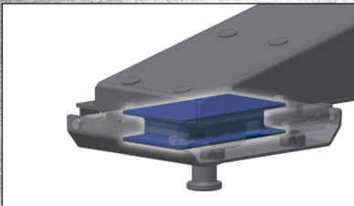
Unique Rubber Shear Spring Absorbs Shock
