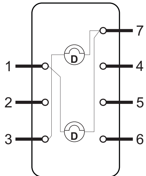
LAMP DIAGRAM
