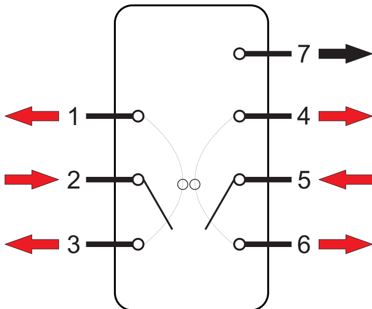
CIRCUIT DIAGRAM
