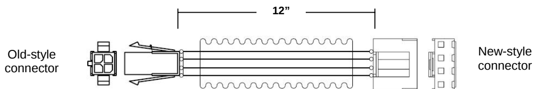
Harness Adapter (P/N: 141-0023012)
