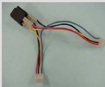
Power Harness 1510000097
