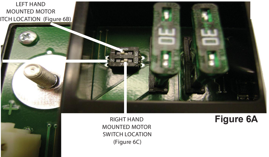
SLIDEOUT MOTOR DIRECTION SWITCHES
