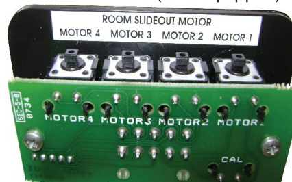
SLIDEOUT ROOM MOTOR BUTTONS
