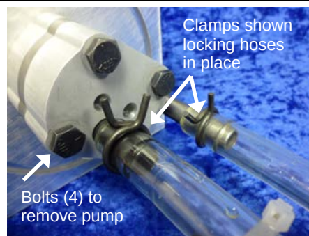
Figure 16 Pump with tubes & clamps
