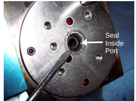
Figure 7 Seal from pump side port hole
