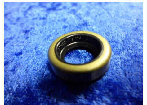
Figure 9 Close-up of the shaft seal (030-1071). Metal side goes in against the port plate.
