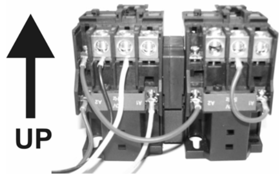
Figure 2 – Floor Mount
