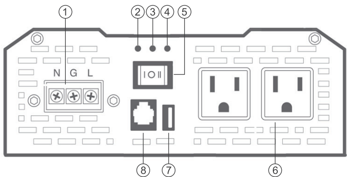
Figure 2: 1000W Inverter
