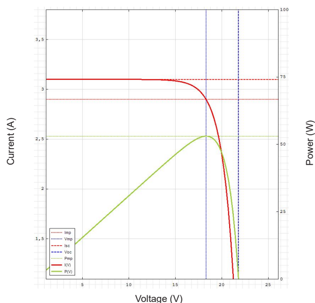
RNG-50D-SS Characteristics Versus Voltage
