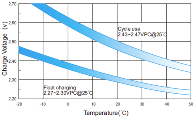
Relationship between Charge Voltage and Temperature
