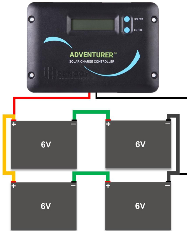
Figure 9.3 Four 6V batteries connected in series – parallel
