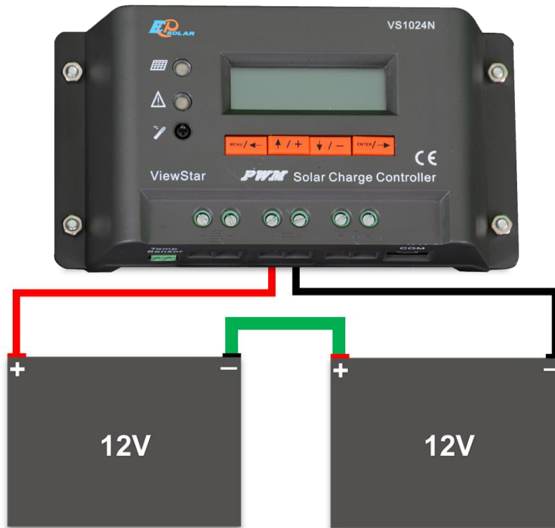
Figure 9.4 Two 12V batteries connected in series
