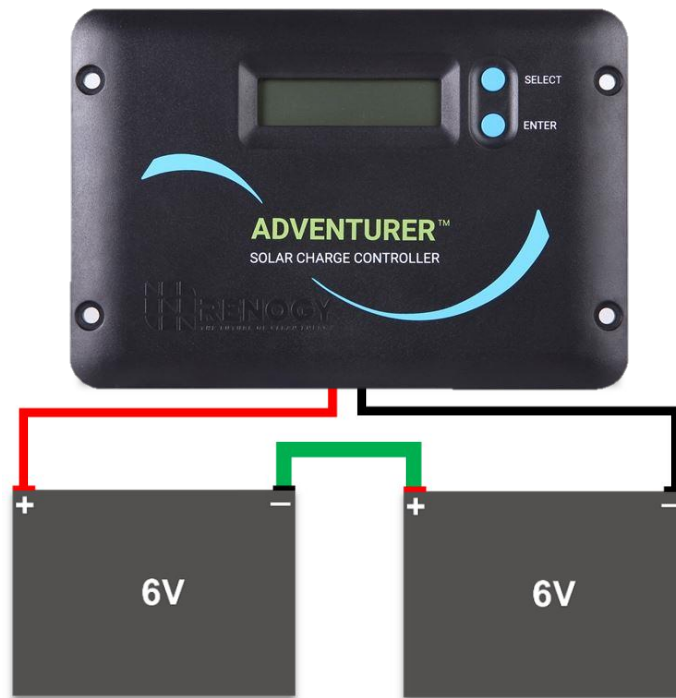
Figure 9.1 Two 6V batteries connected in series
