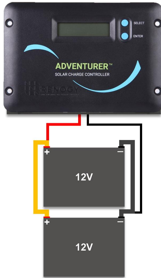
Figure 9.2 Two 12V batteries connected in parallel
