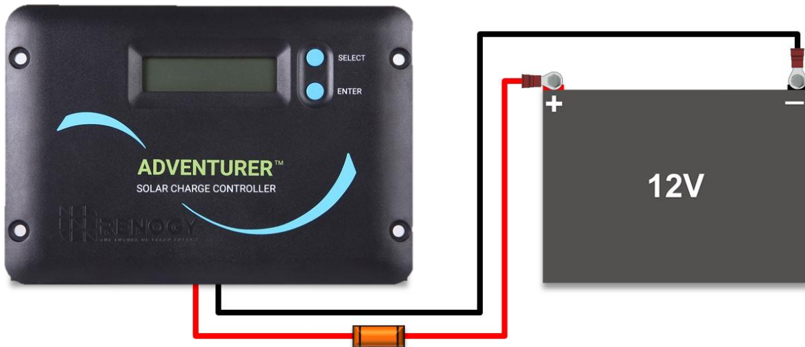
Figure 6.1 Charge controller connected to a 12V battery
