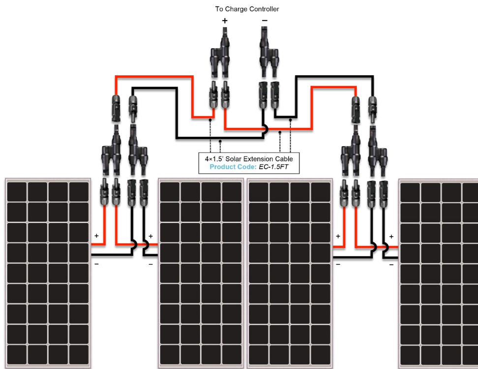
Figure 8.5 Four RNG-100D Panels in parallel
