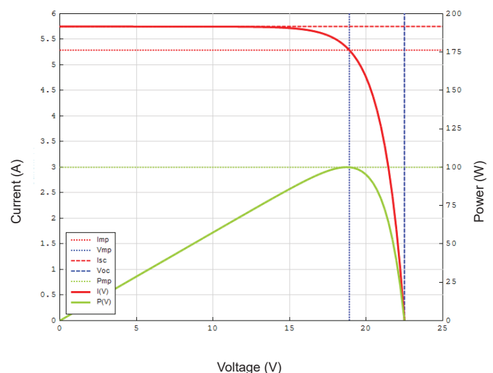
RNG-100MB Characteristics Versus Voltage
