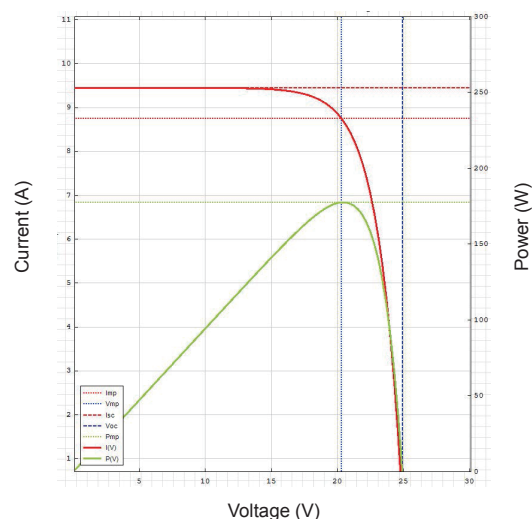
RNG-160DB-H Characteristics Versus Voltage
