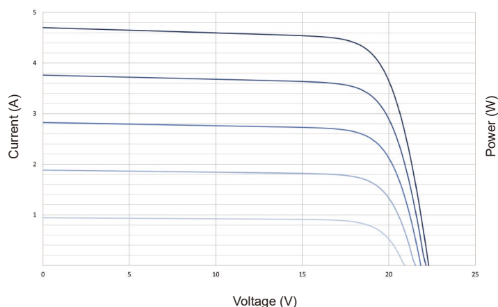
RNG-80D-SS Characteristics Versus Voltage
