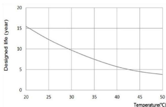
Designed life Vs temperature
